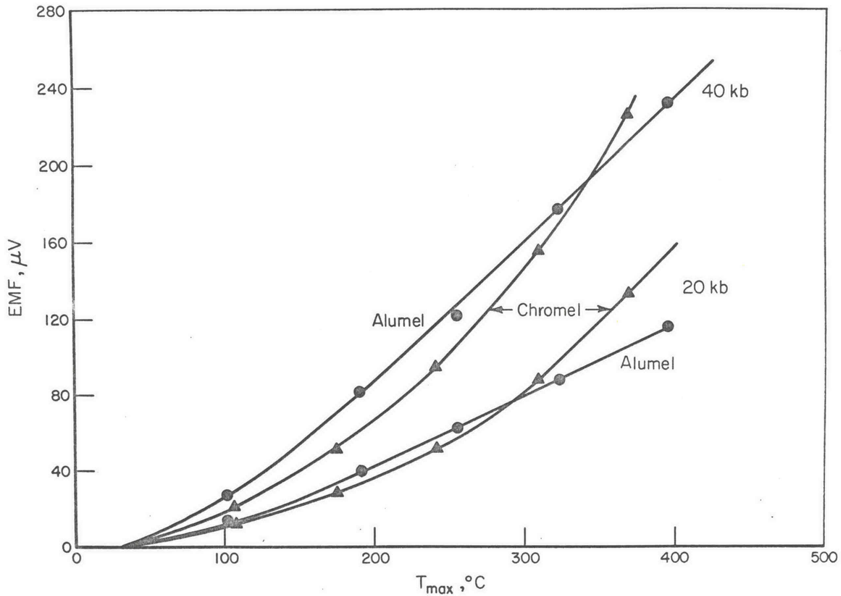
PRESSURE EMF VERSUS TEMPERATURE CHROMEL-ALUMEL Cold + ; hot -
